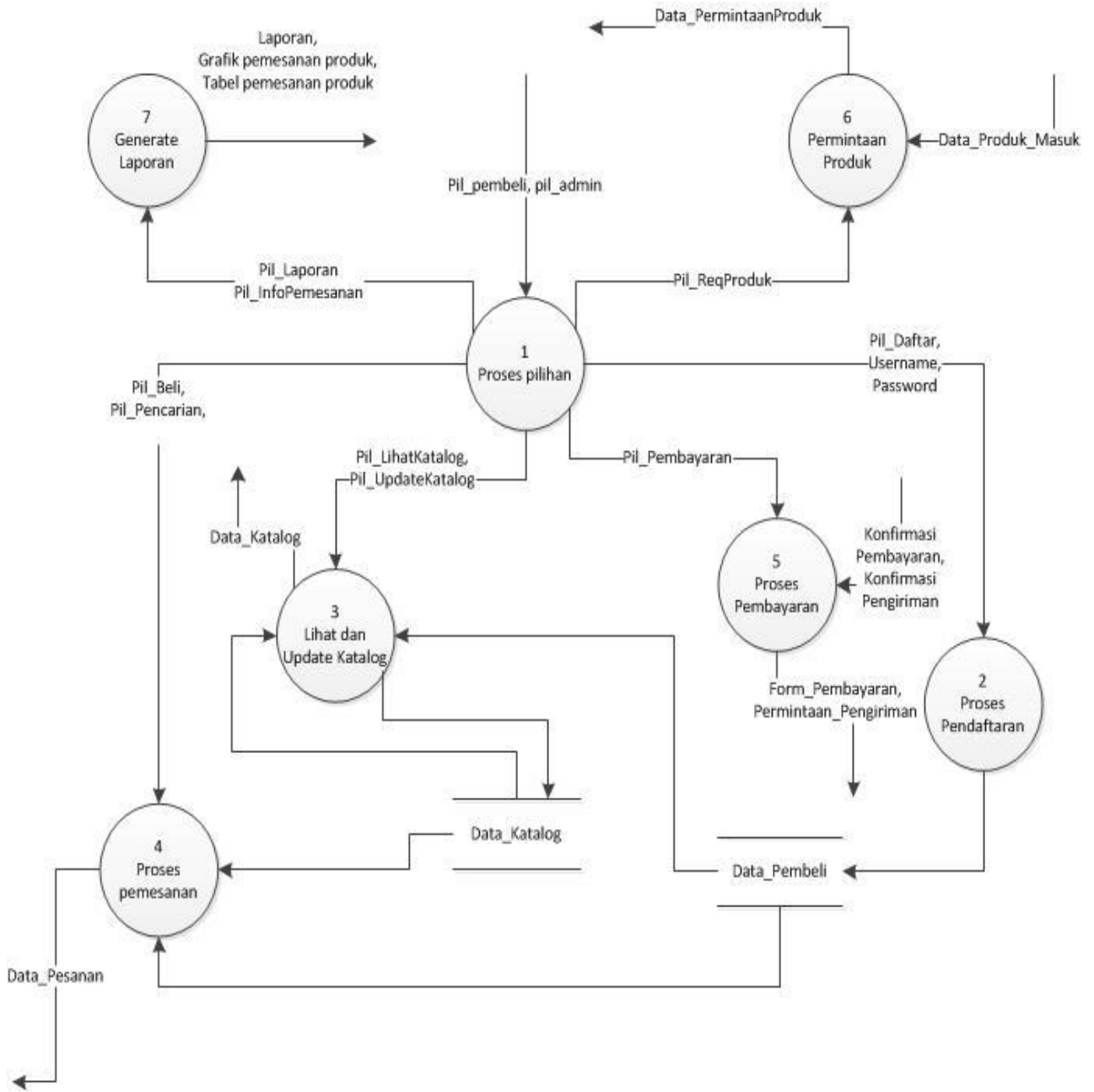
Gambar 3. Diagram Level 1 SI Transaksi SMM
